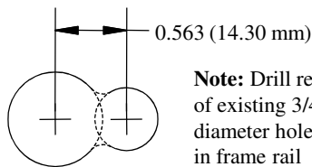
Figure 1: Access hole modification to allow pull wiring of block and carriage bolt
